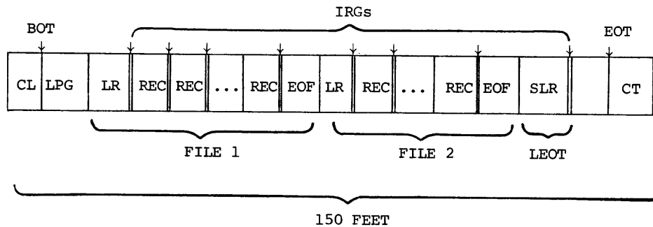
Figure 6-1 Structure of Cassette Tape
