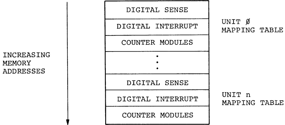
Figure 14-1A Mapping Table Format
